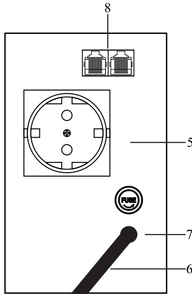
REAR PANEL VIEW UPS CT382B
