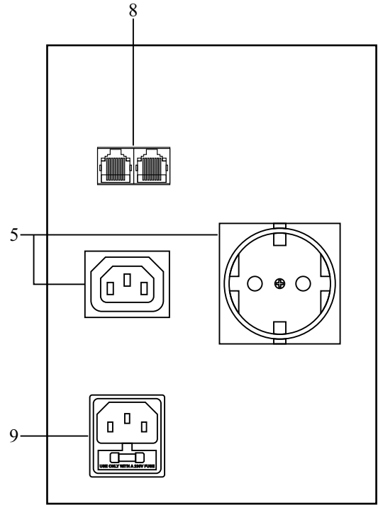
REAR PANEL VIEW UPS CT682B
