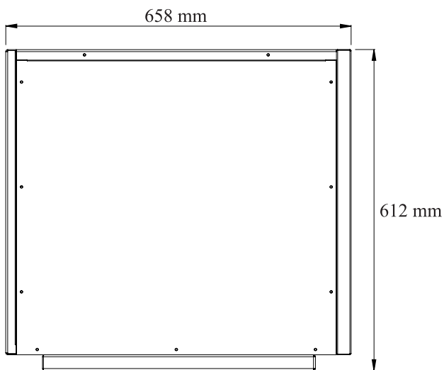
Tampak Samping
